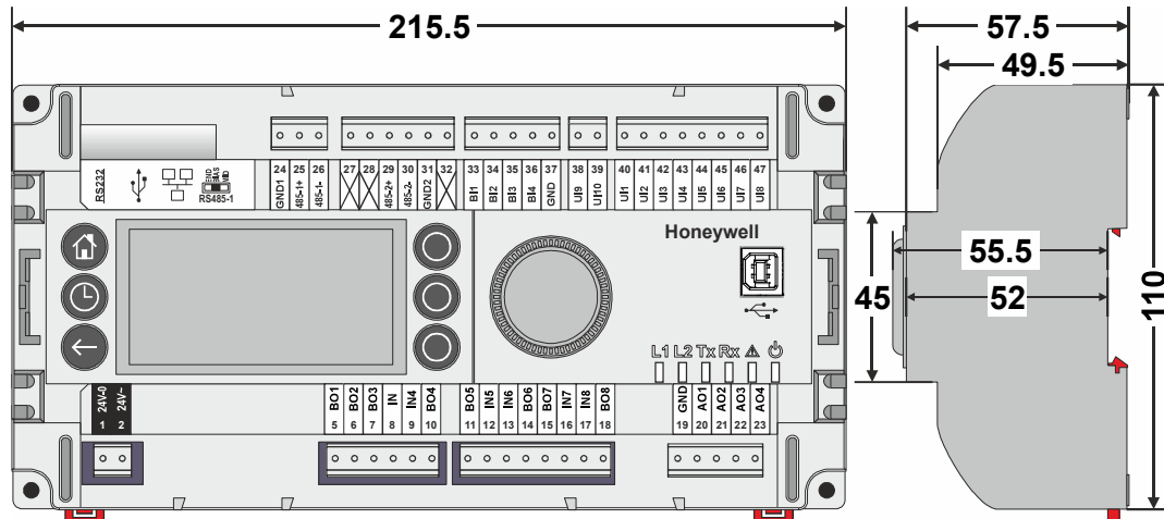
Fig. 9. MVCweb Controller with built-in HMI, dimensions (in mm)
