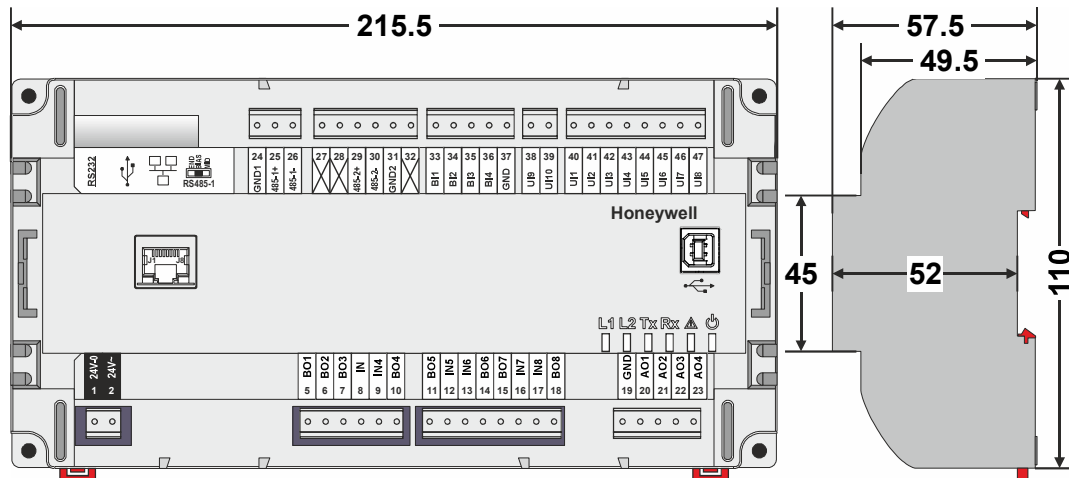
Fig. 10. MVCweb Controller with RJ45 socket for connection of MVC-2000HMI-A External HMI, dimensions (in mm)
