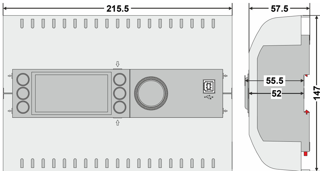
Fig. 11. MVCweb Controller with built-in HMI (with MVC-80-AC1), dimensions (in mm)
