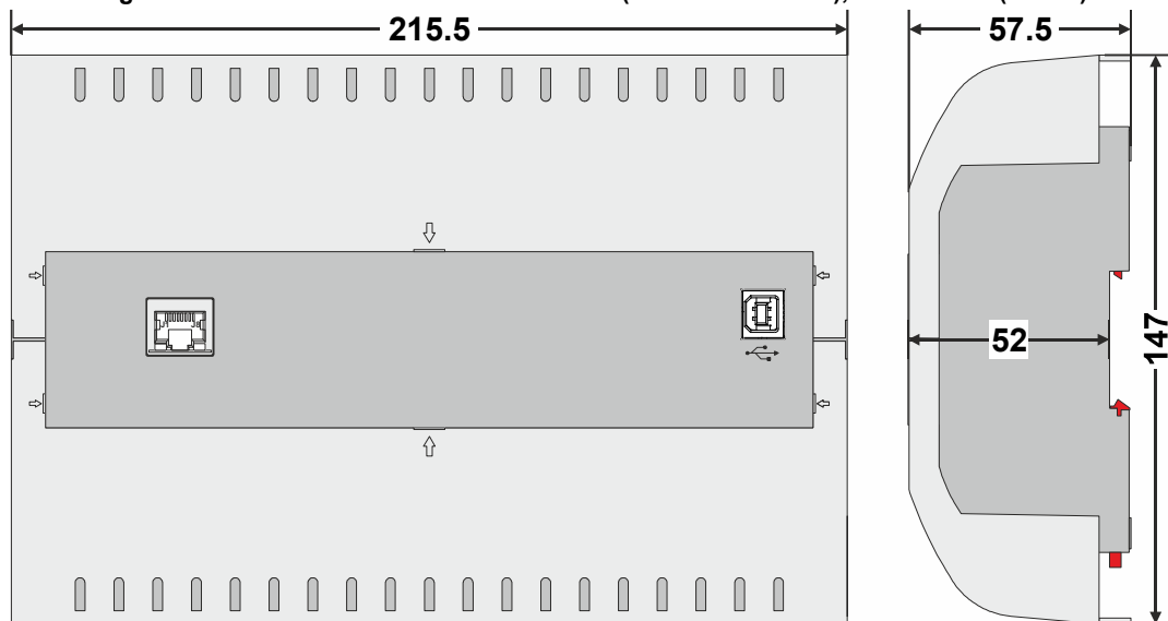
Fig. 12. MVCweb Controller with RJ45 socket for MVC-2000HMI-A External HMI (with MVC-80-AC1), dimensions (in mm)
